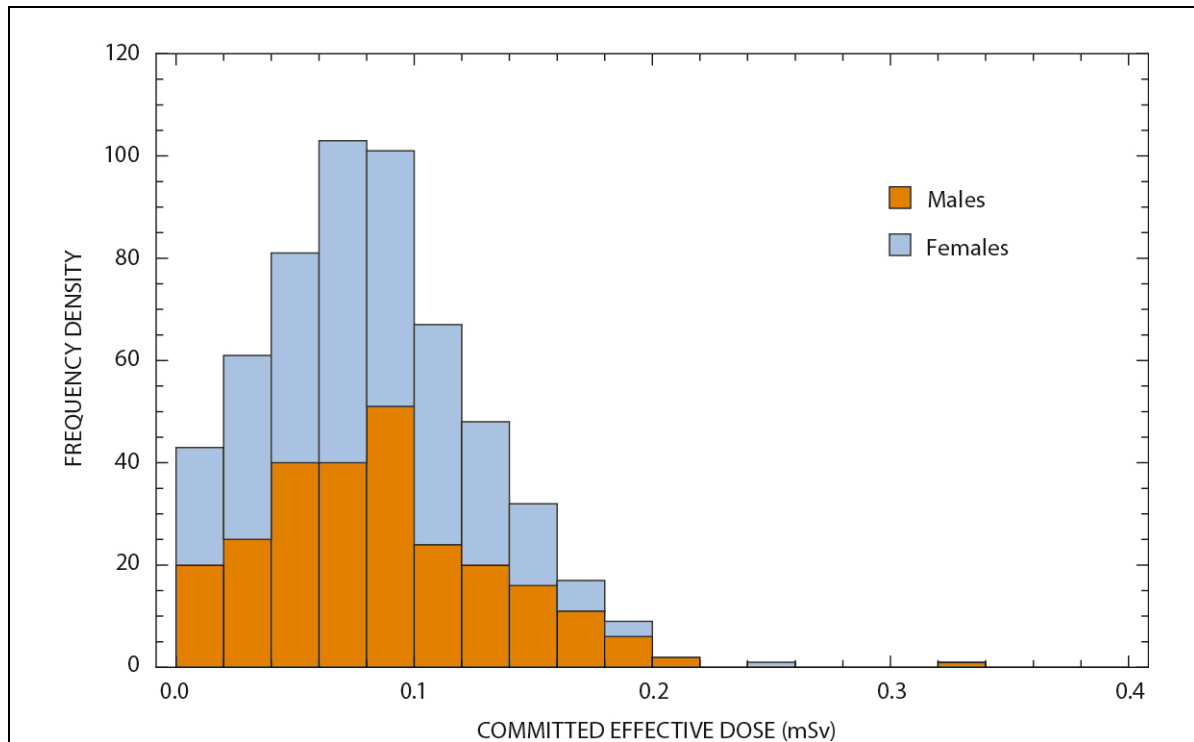
Figure II. The estimated committed effective dose to adult residents of Minamisoma City based on WBC measurements conducted 110–140 days after the FDNPS accident assuming early intake of caesium radionuclides [H3]
